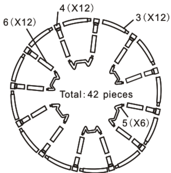
➤10', 12',13',14',15',16' Trampoline( 6Legs )
