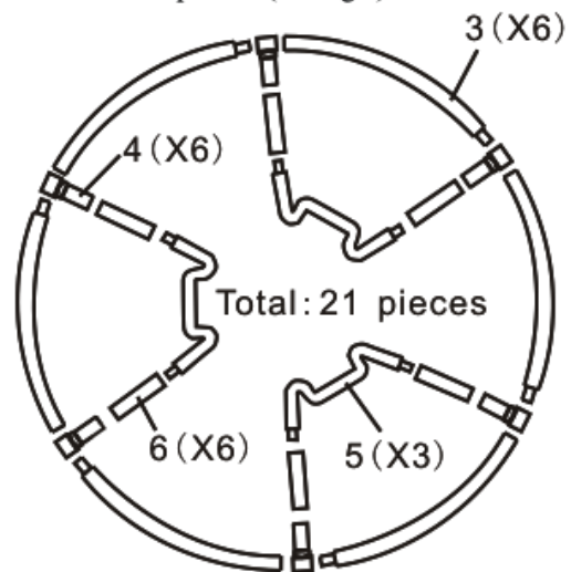
➤8', 10' Trampoline ( 3 Legs )
