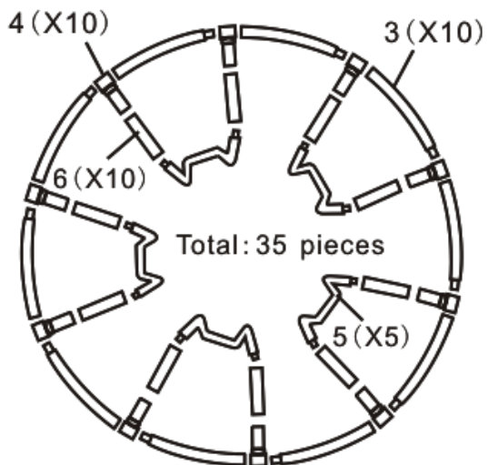
➤ 10',12',13',14',15',16' Trampoline( 5 Legs )
